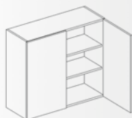
W 80 SHG 800X720X288
